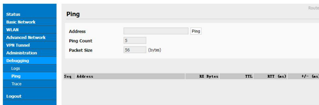
Figure 3-27 Ping GUI
