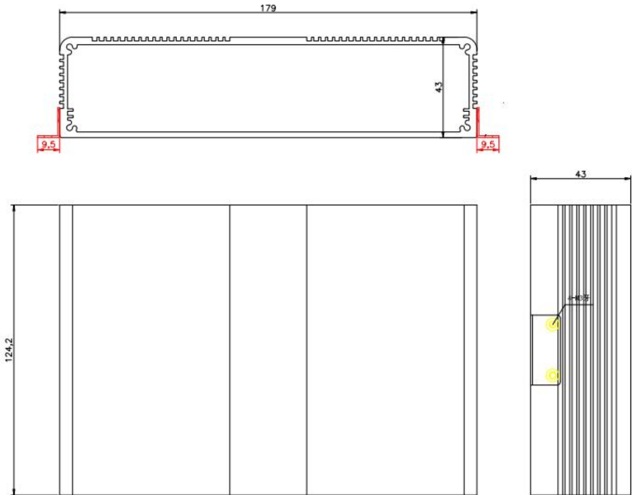
Figure 1-2 G930 Series Router Dimension
